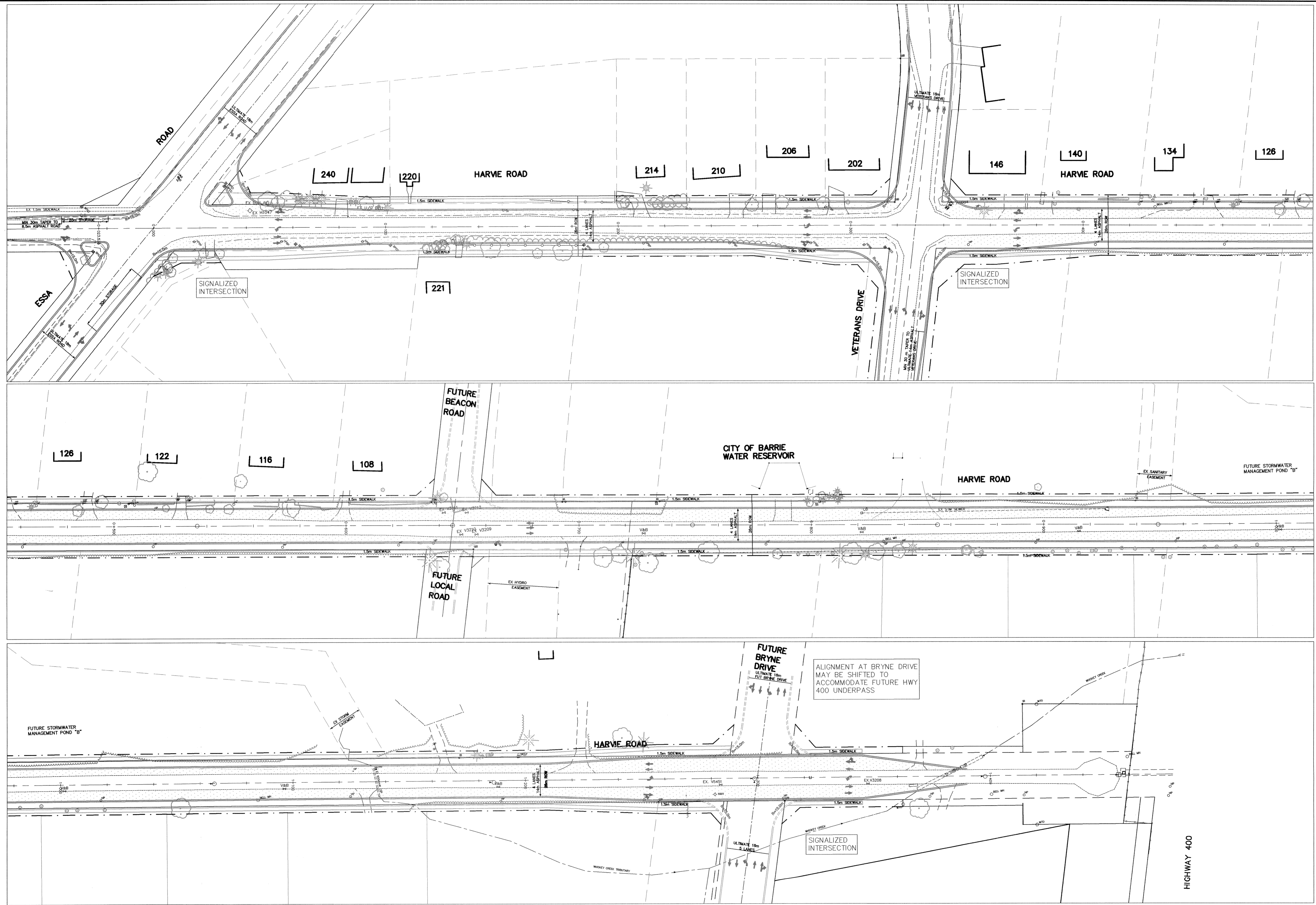
FIGURE 4A ALTERNATIVE 4A FOUR LANES, URBAN SECTION WITH OPERATIONAL IMPROVEMENTS (REALIGNMENT AT VETERANS DRIVE) SCALE 1:750
