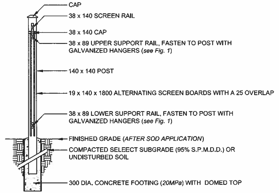
SECTION B-B
