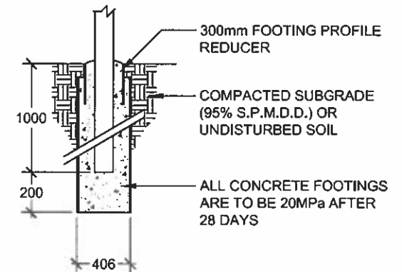
FOOTING DETAIL
