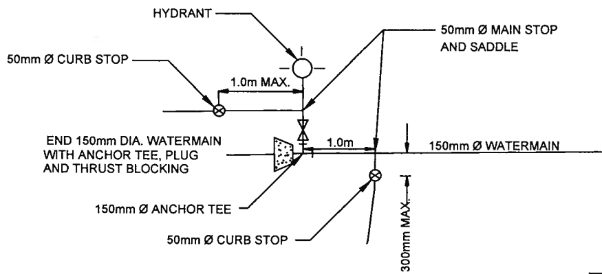
DETAIL "A"
