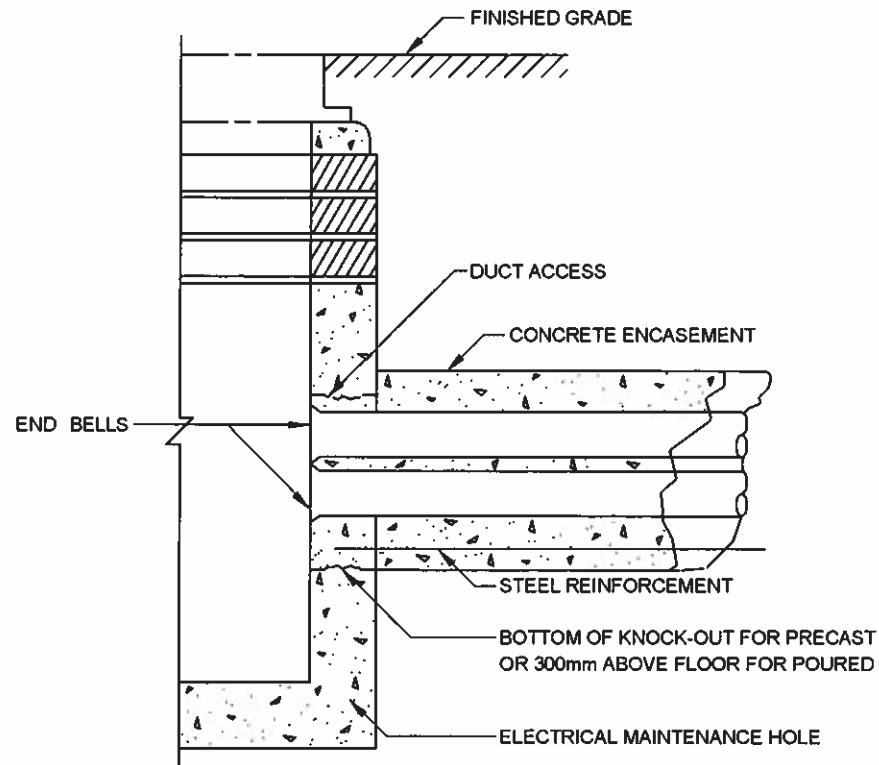
RIGID DUCTS, CONCRETE ENCASED
