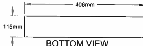
BOTTOM VIEW
