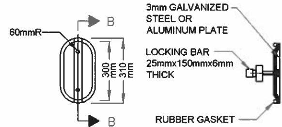
HAND HOLE COVER DETAIL 'B'
