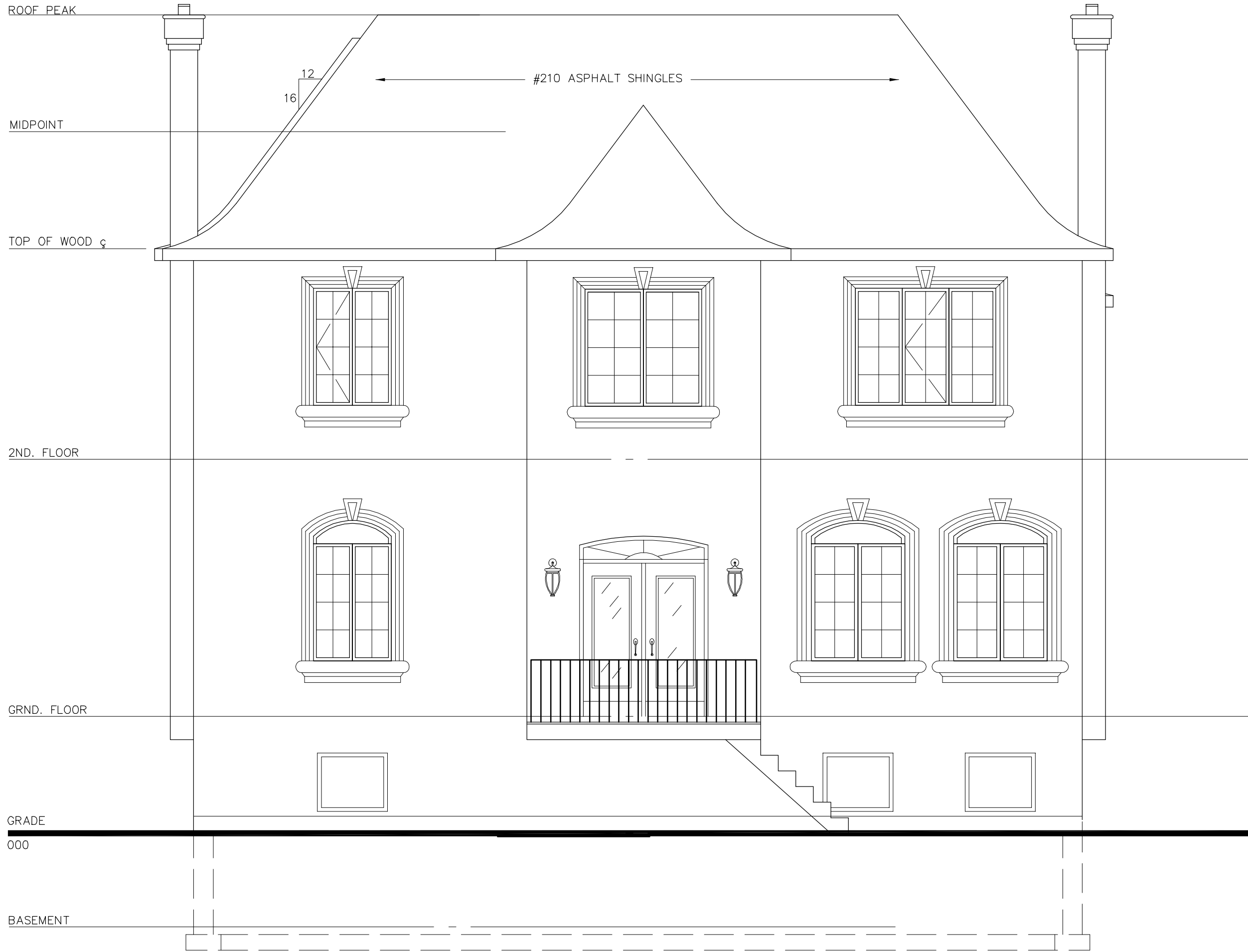
REAR ELEVATION
