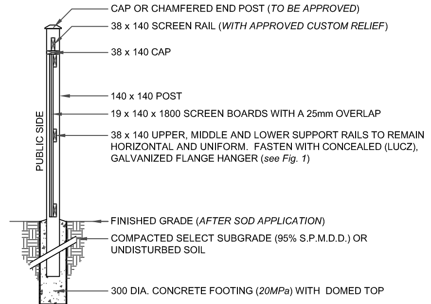
SECTION B-B
