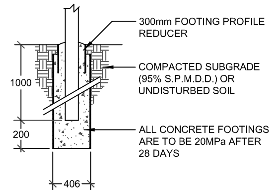
FOOTING DETAIL
