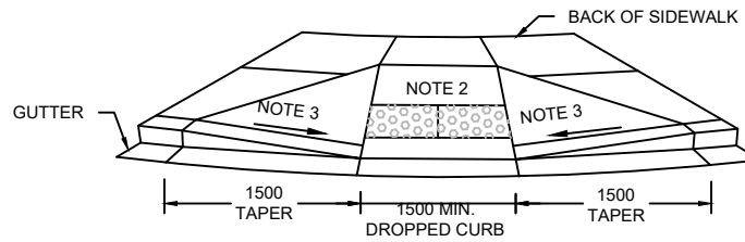
RAMP ELEVATION
