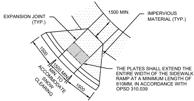
RAMP PLAN
