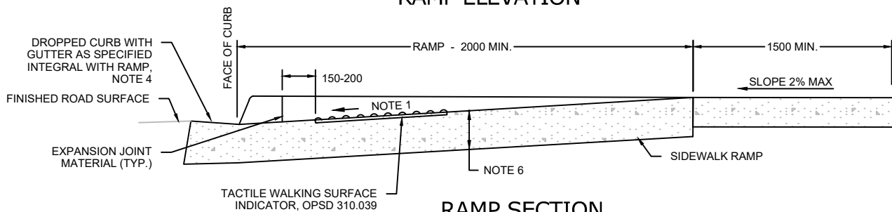
RAMP SECTION
