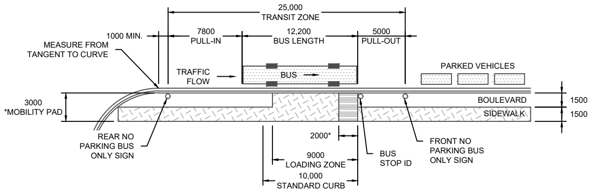
FAR-SIDE BUS STOP WITH CURB, BOULEVARD, SIDEWALK
