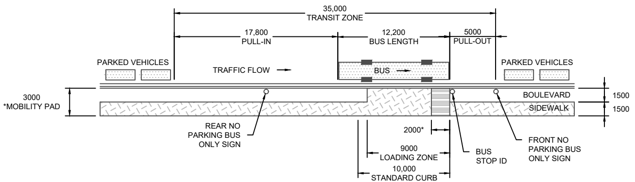
MID-BLOCK BUS STOP WITH CURB, BOULEVARD, SIDEWALK
