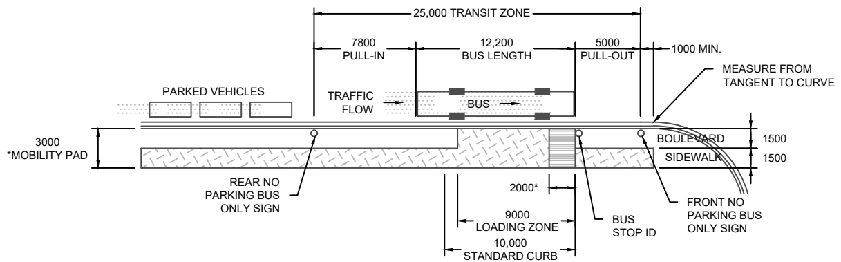
NEAR-SIDE BUS STOP WITH CURB, BOULEVARD, SIDEWALK
