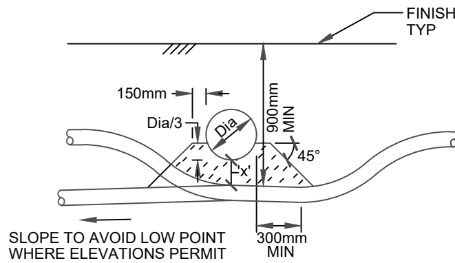
CROSSING UNDER UTILITY
