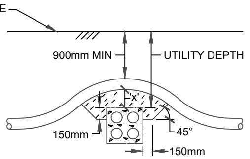
CROSSING OVER CONCRETE ENCASED UTILITY
