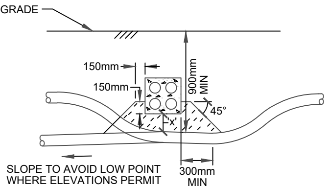
CROSSING UNDER CONCRETE ENCASED UTILITY
