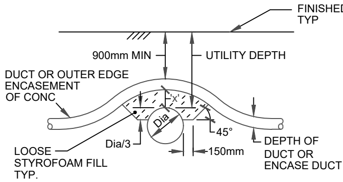
CROSSING OVER UTILITY
