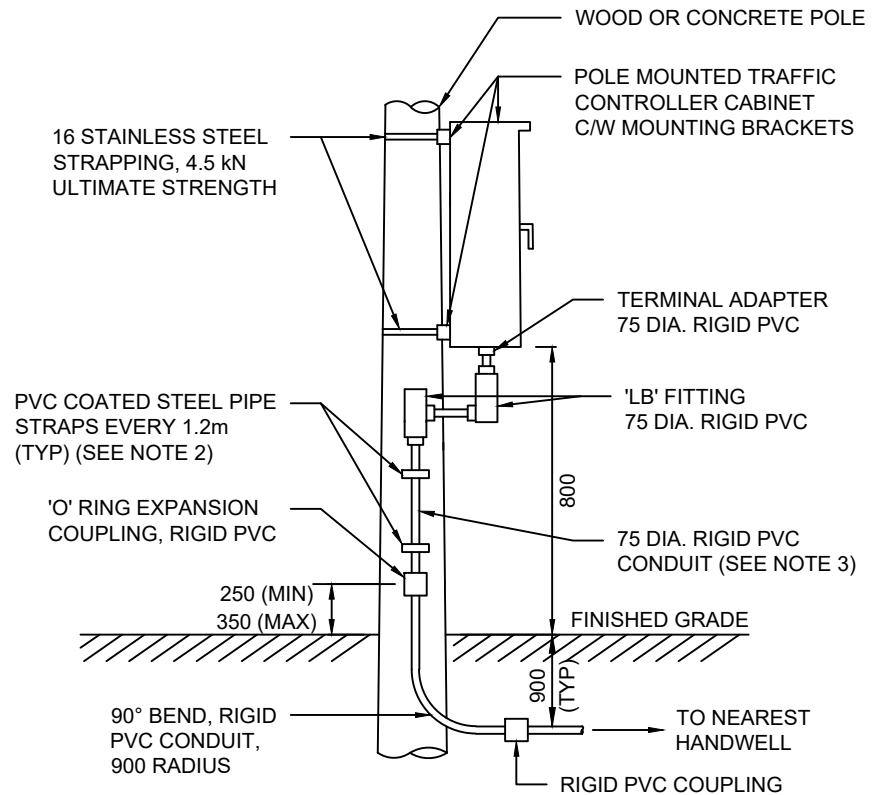
UNDERGROUND INSTALLATION
