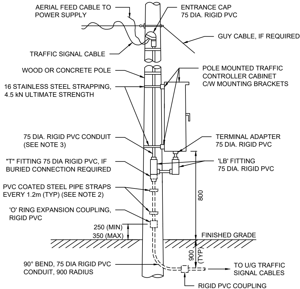
AERIAL INSTALLATION
