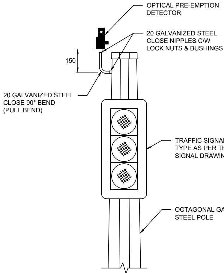
POLE MOUNTING
