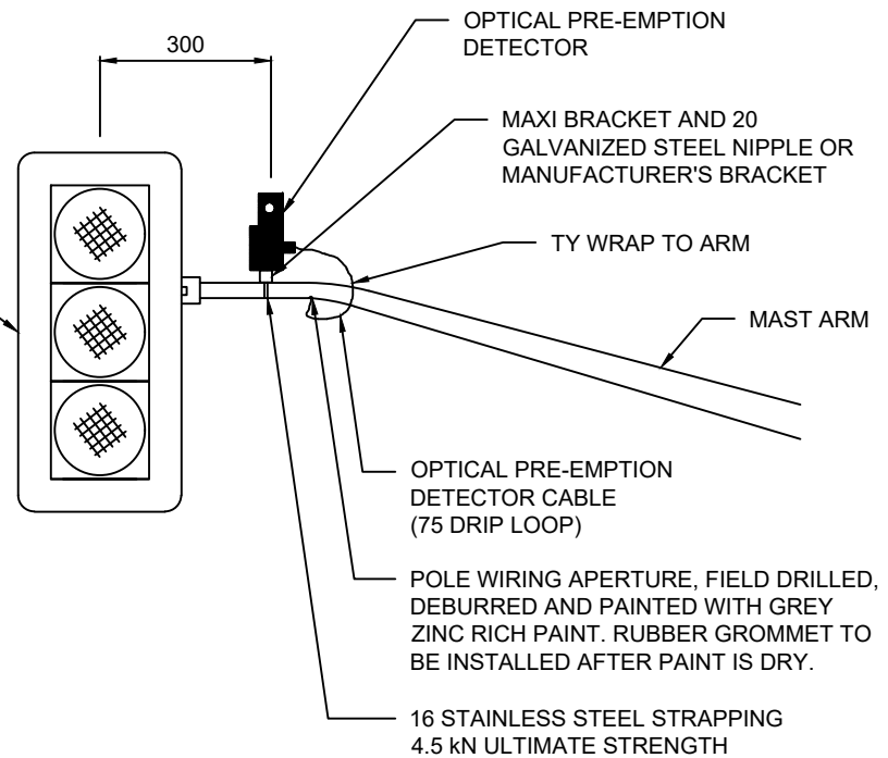
MAST ARM MOUNTING
