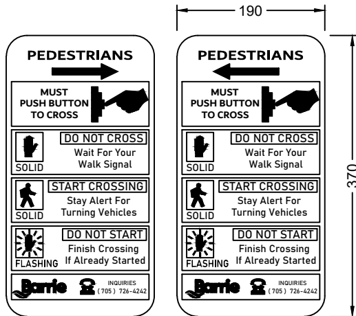
PEDESTRIAN PUSHBUTTON SIGNS DETAIL 'B'
