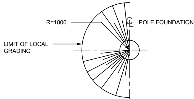
TYPICAL PLAN
