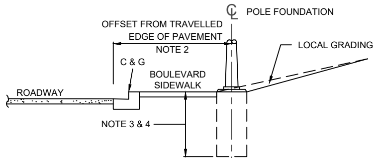
POLE FOUNDATION ADJACENT TO SIDEWALK
