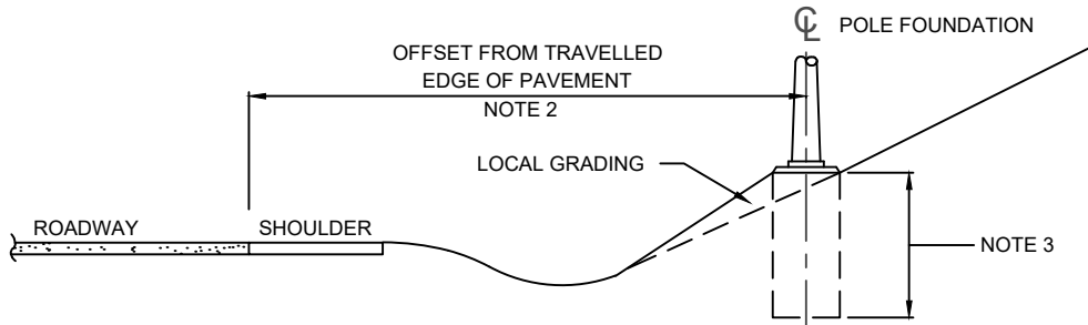
POLE FOUNDATION IN CUT
