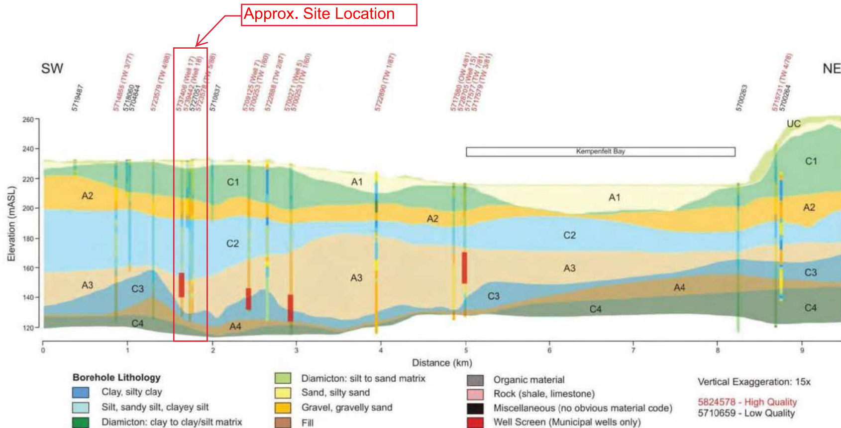
Figure 2-22: Southwest to northeast cross-section through the City of Barrie (AquaResource et al. , 2011).
