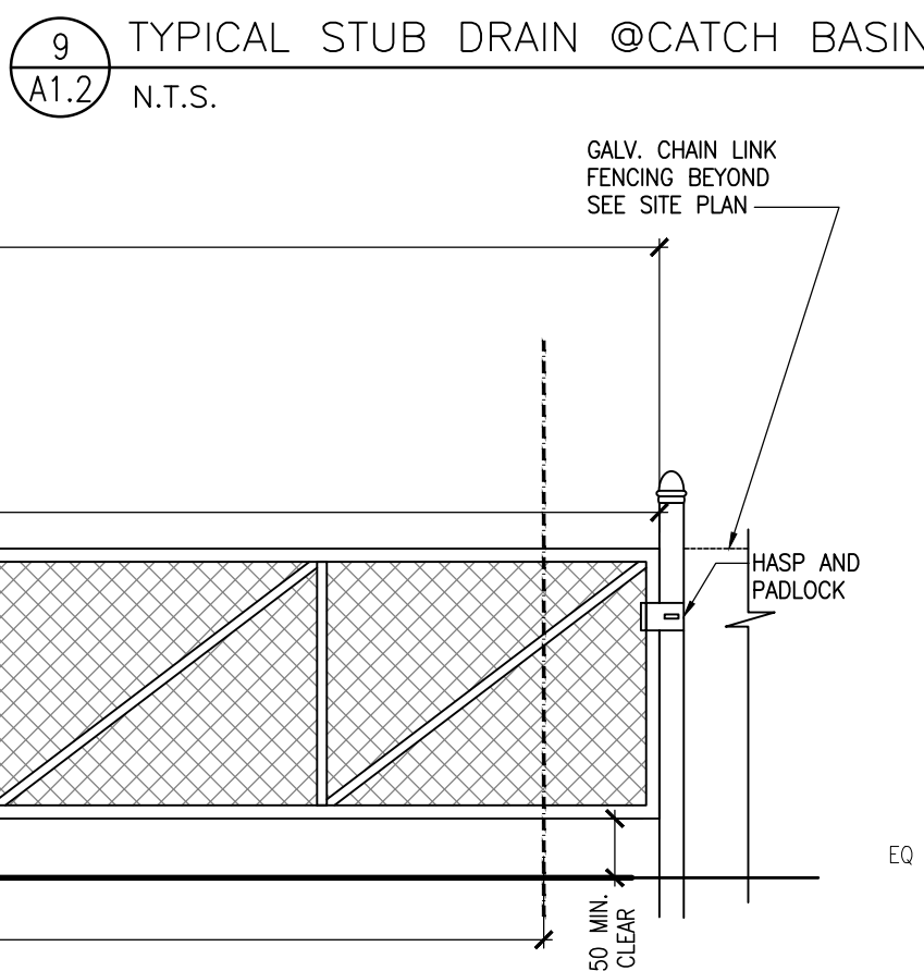
9 TYPICAL STUB DRAIN @CATCH BASIN
