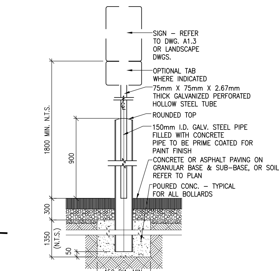
15 SIGNAGE BOLLARD TYPE "B1" DETAIL
