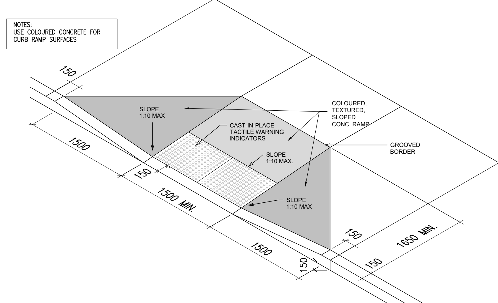
6A CURB RAMP (AXONOMETRIC VIEW)
