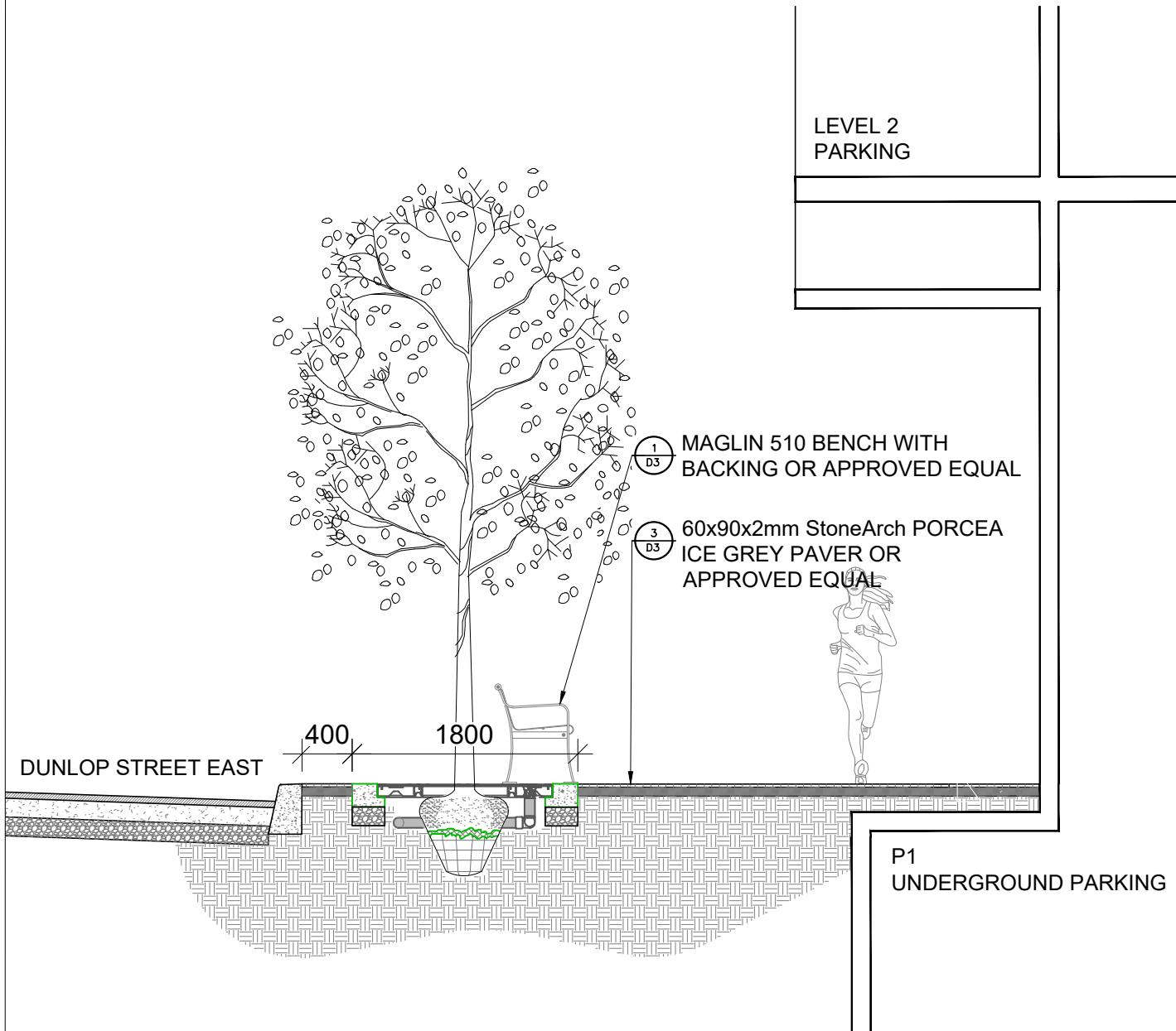
2 DUNLOP STREET CROSS SECTION
