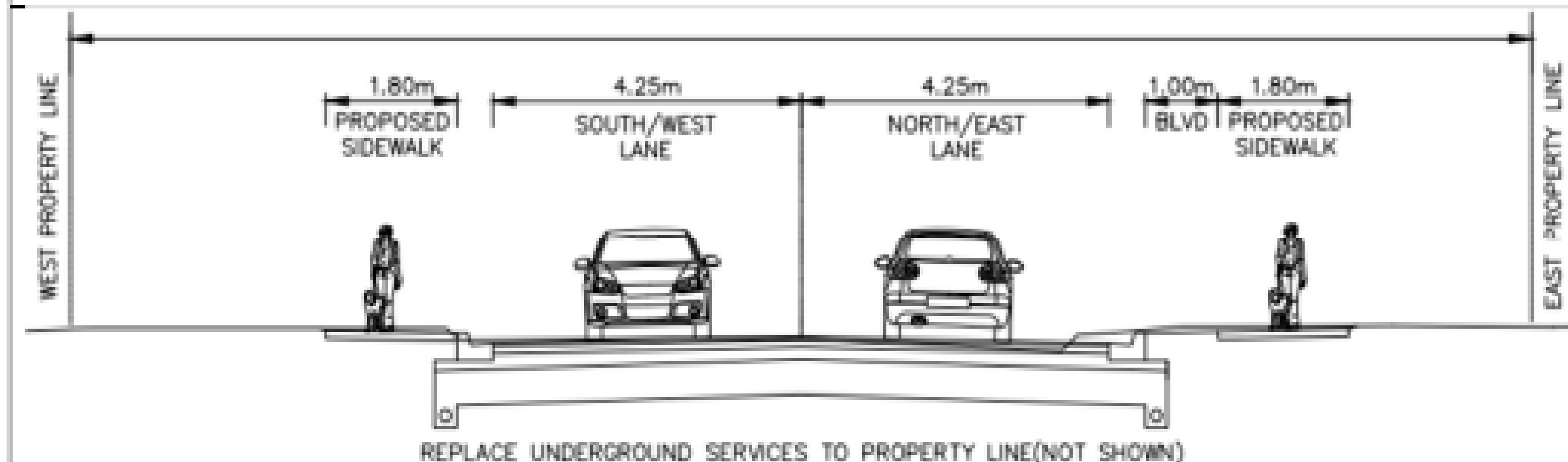
PROPOSED DUNDONALD ST. FROM THERESA STREET TO 52 DUNDONALD ST.
