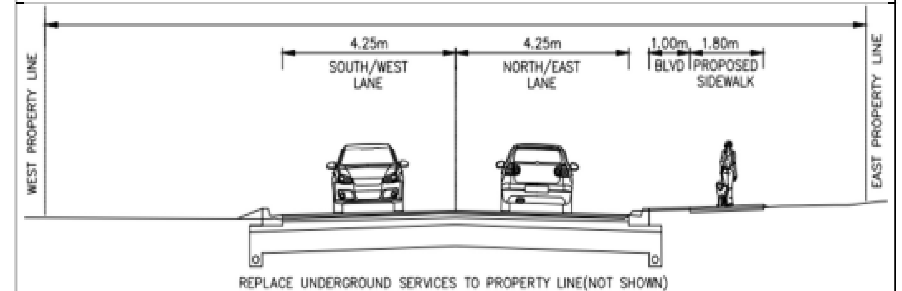
PROPOSED DUNDONALD ST. FROM 52 DUNDONALD STREET TO EUGENIA ST.
