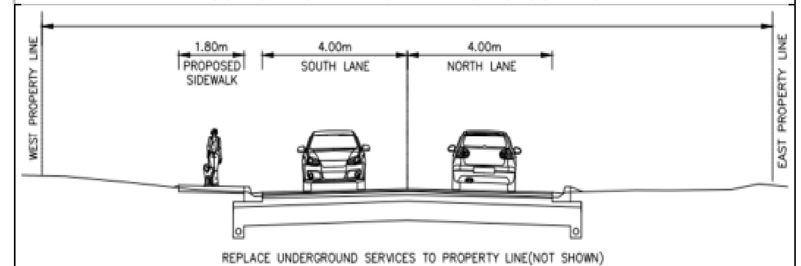
DUCKWORTH STREET FROM AMELIA ST. TO EUGENIA ST.
