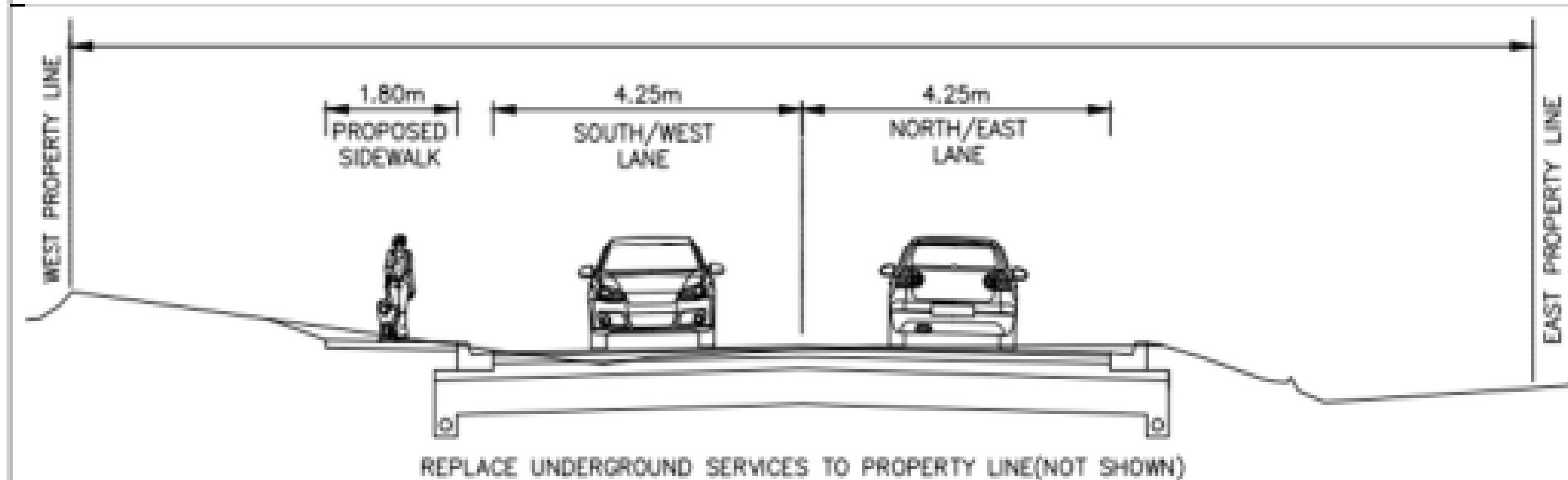
PROPOSED DUNDONALD ST. FROM COLLIER STREET TO THERESA ST.
