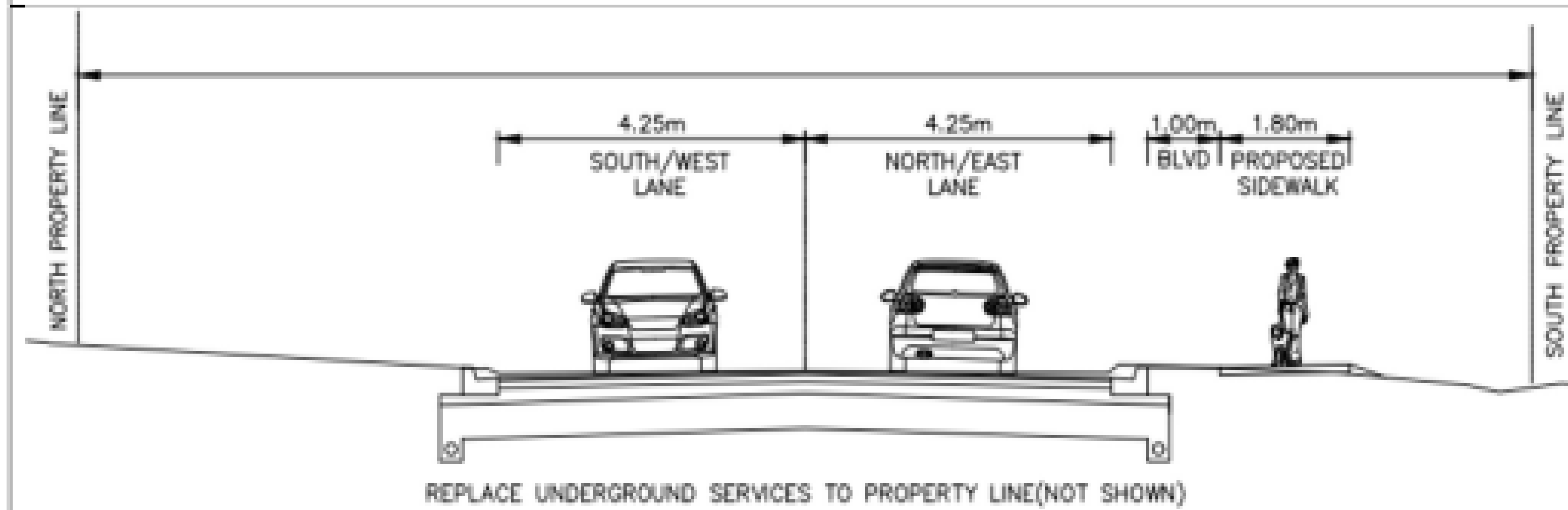
PROPOSED AMELIA ST. FROM DUNDONALD STREET TO DUCKWORTH ST.
