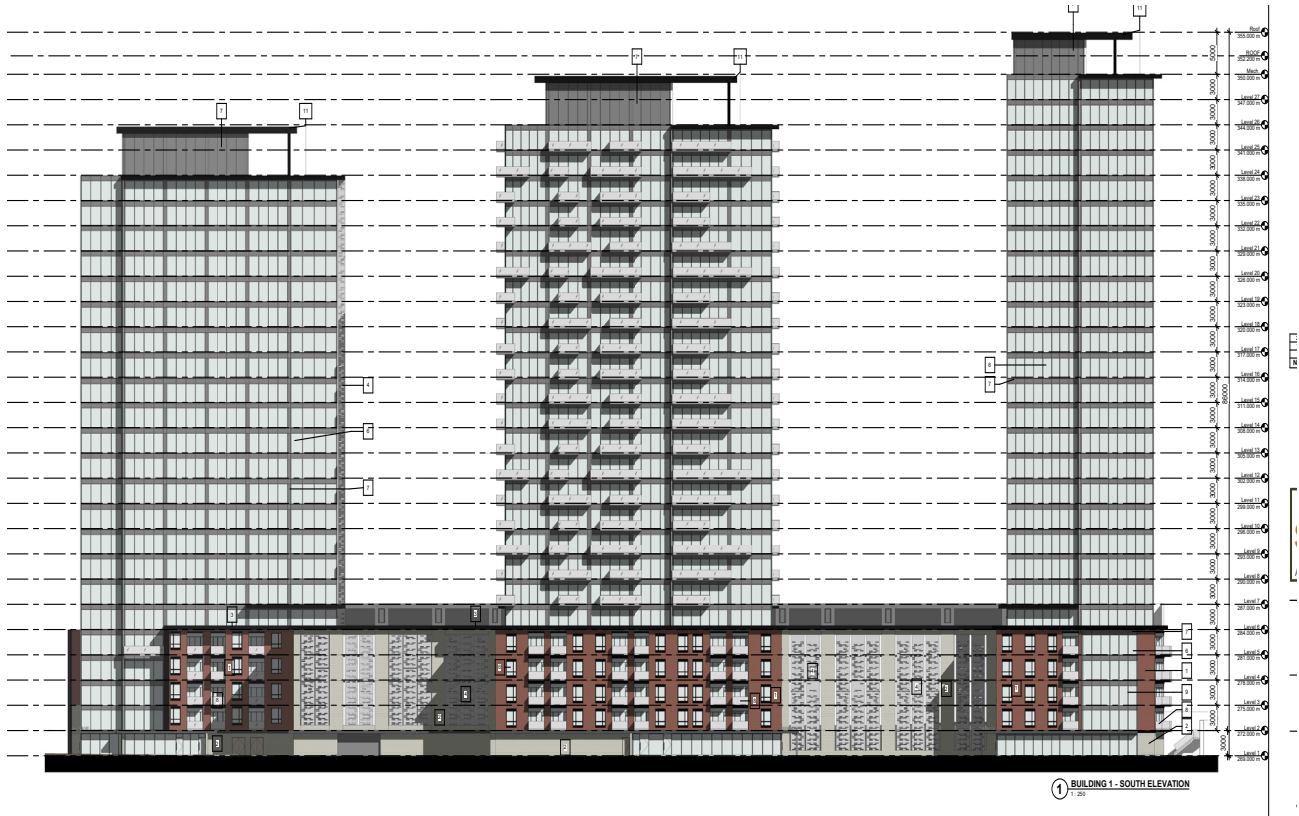
Figure 9.4 Elevation for Building 1,2,3 prepared by SRM Architects.
