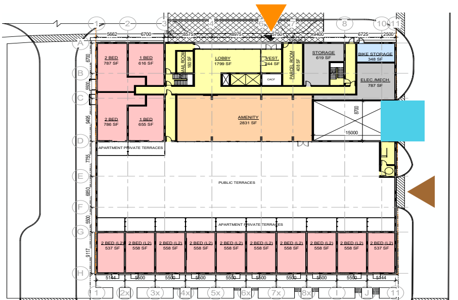
Figure 6.5 Building 4 Ground Level Plan illustrating building frontage and access points
