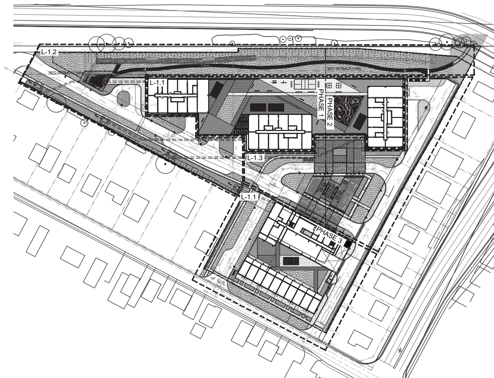
Figure 10.1 Overall Landscape plan illustrating the proposed roof top amenities, at-grade amenity and landscaped areas.
