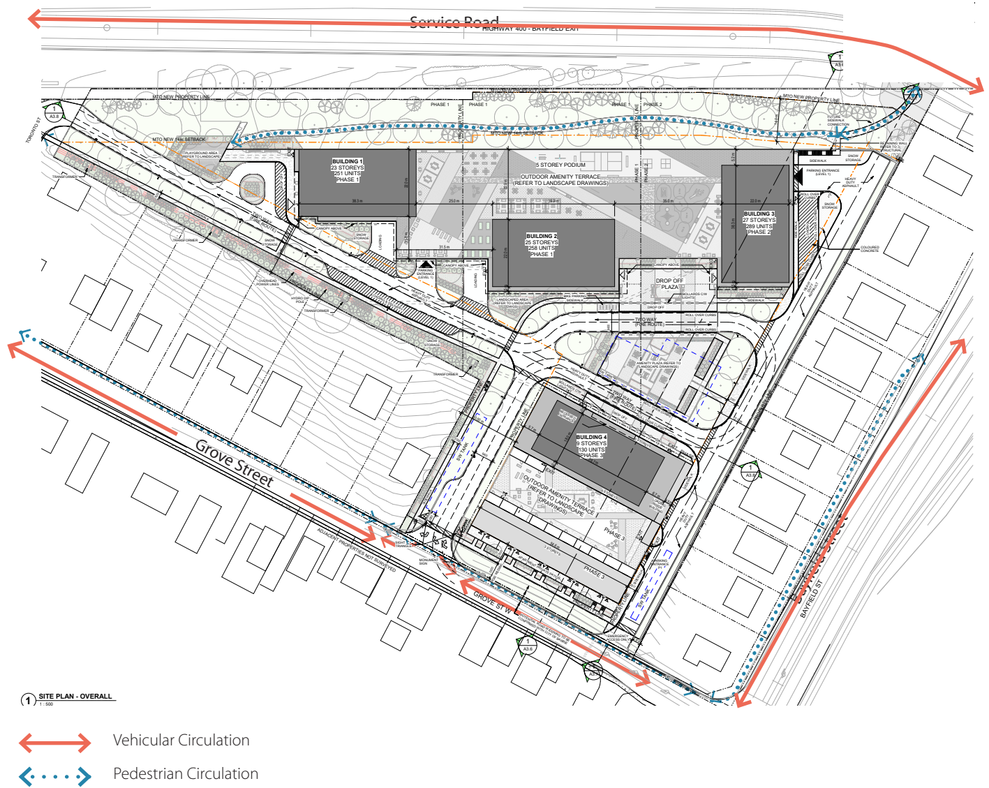
Figure 7.2 Pedestrian circulation and location of main building entrances. Site plan by SRM Architects.
