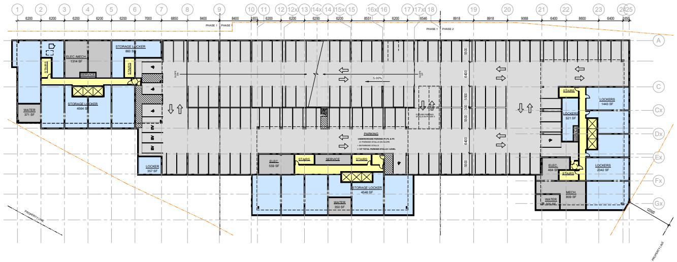
Figure 8.3 Building 1,2,3, Underground parking level.
