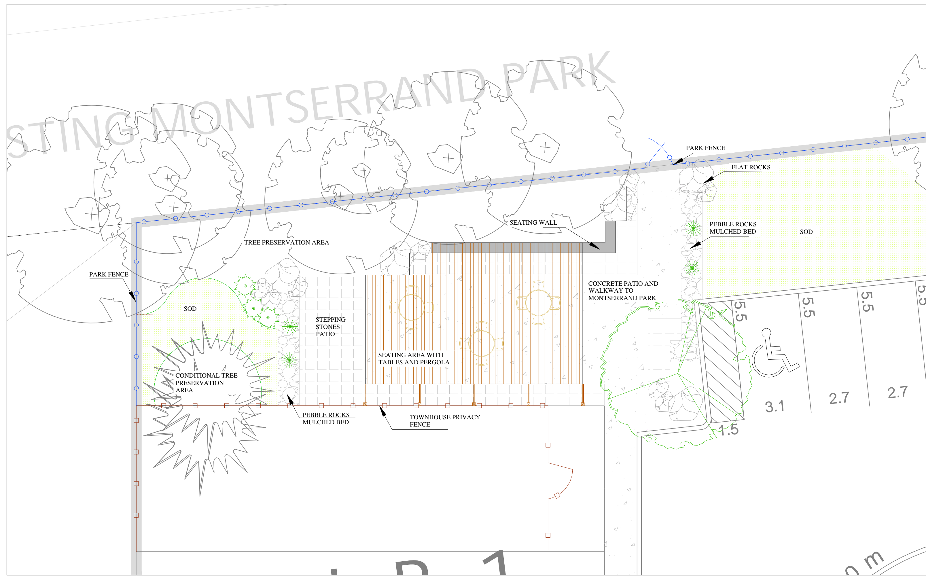
AMENITY AREA CONCEPT PLAN
