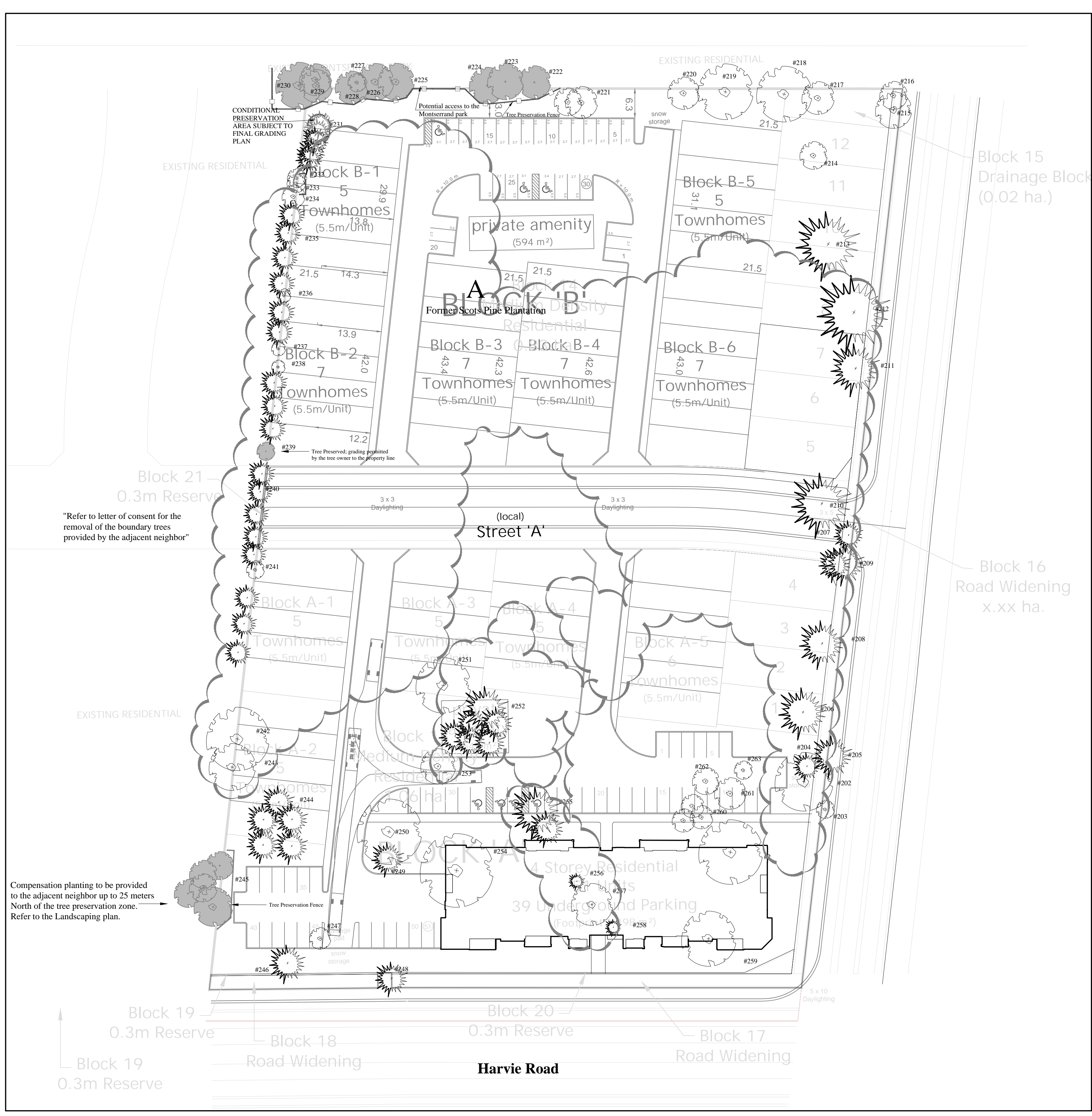
TREE PRESERVATION PLAN 1:500
