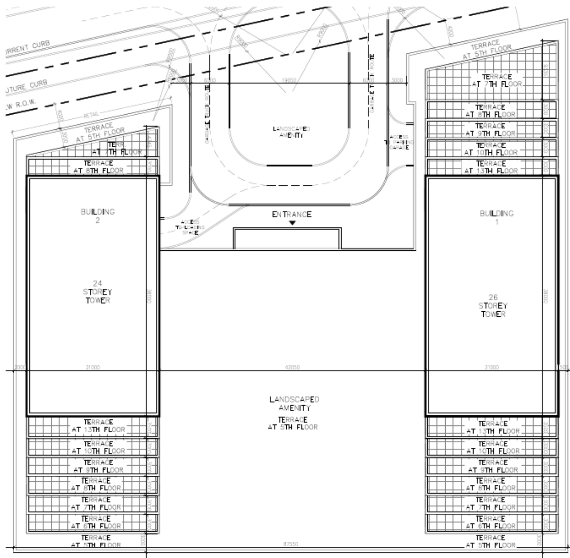
Figure 1 - 17 Jacobs Terrace –Site Plan (Courtesy of MARK ZWICKER – architectural team)
