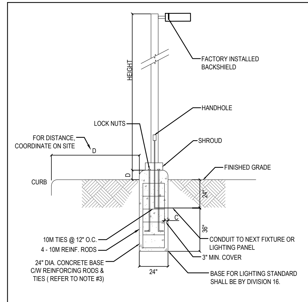
TYPICAL LIGHT POST FULL CUT-OFF LIGHTING SCALE: N.T.S
