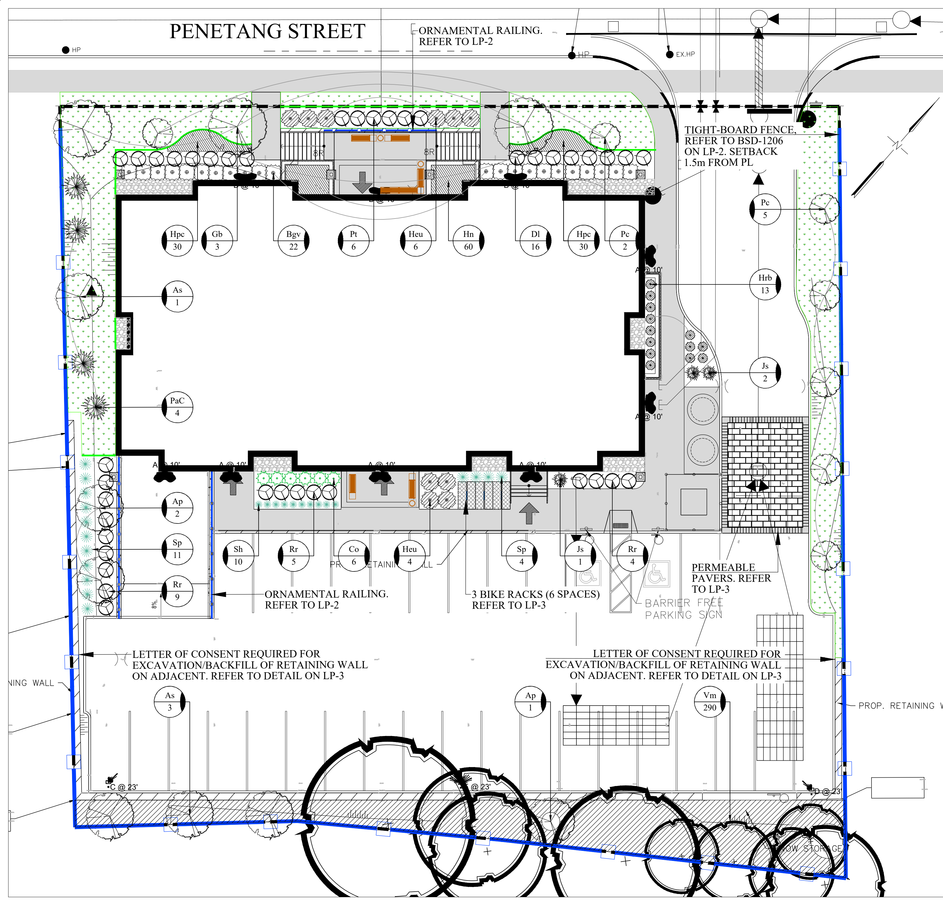
LANDSCAPE PLAN SCALE 1 : 150
