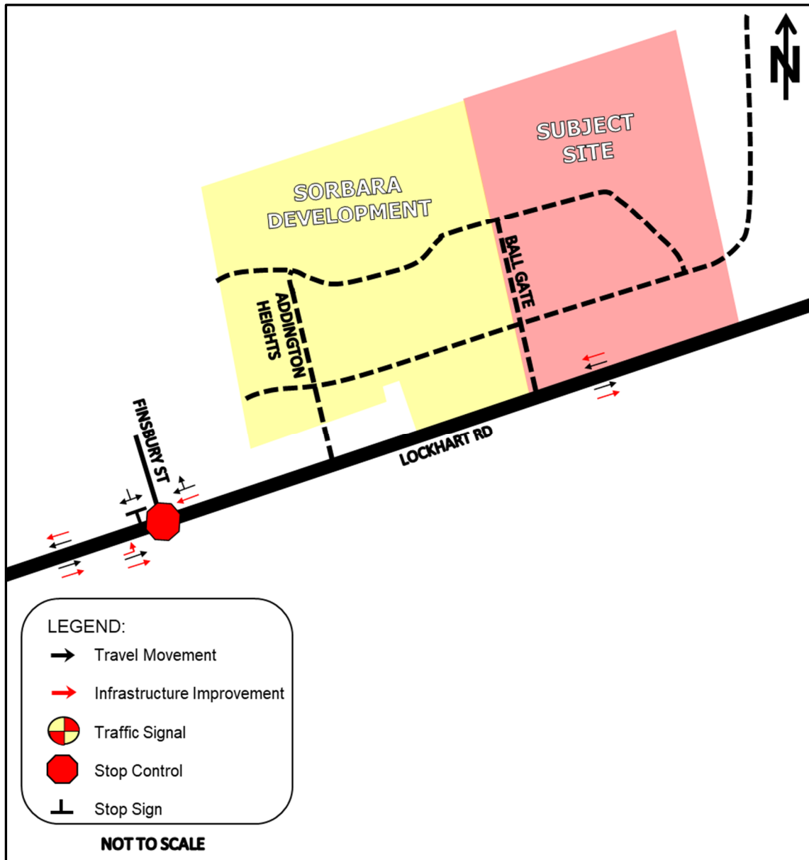
Figure 3 – Future Lane Configuration within Study Area
