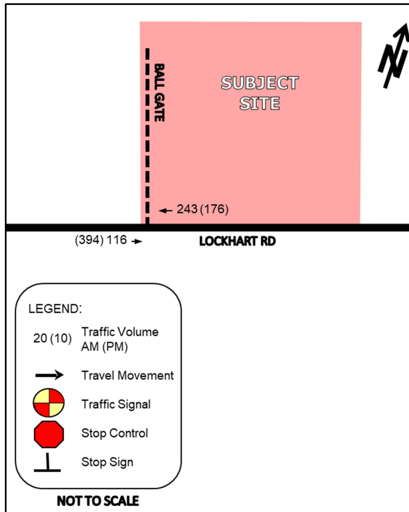
Figure 14 – Existing (2021) Traffic Volumes
