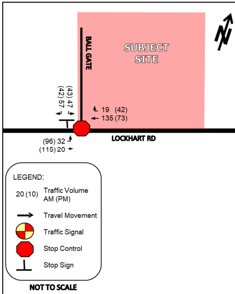
Figure 12 – Total Adjacent Development Traffic (2025)
