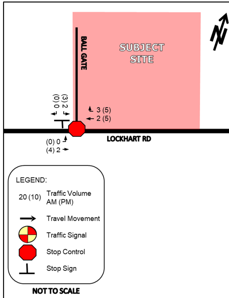
Figure 11 – VDH Development Traffic Assignment (2031 / 2035)
