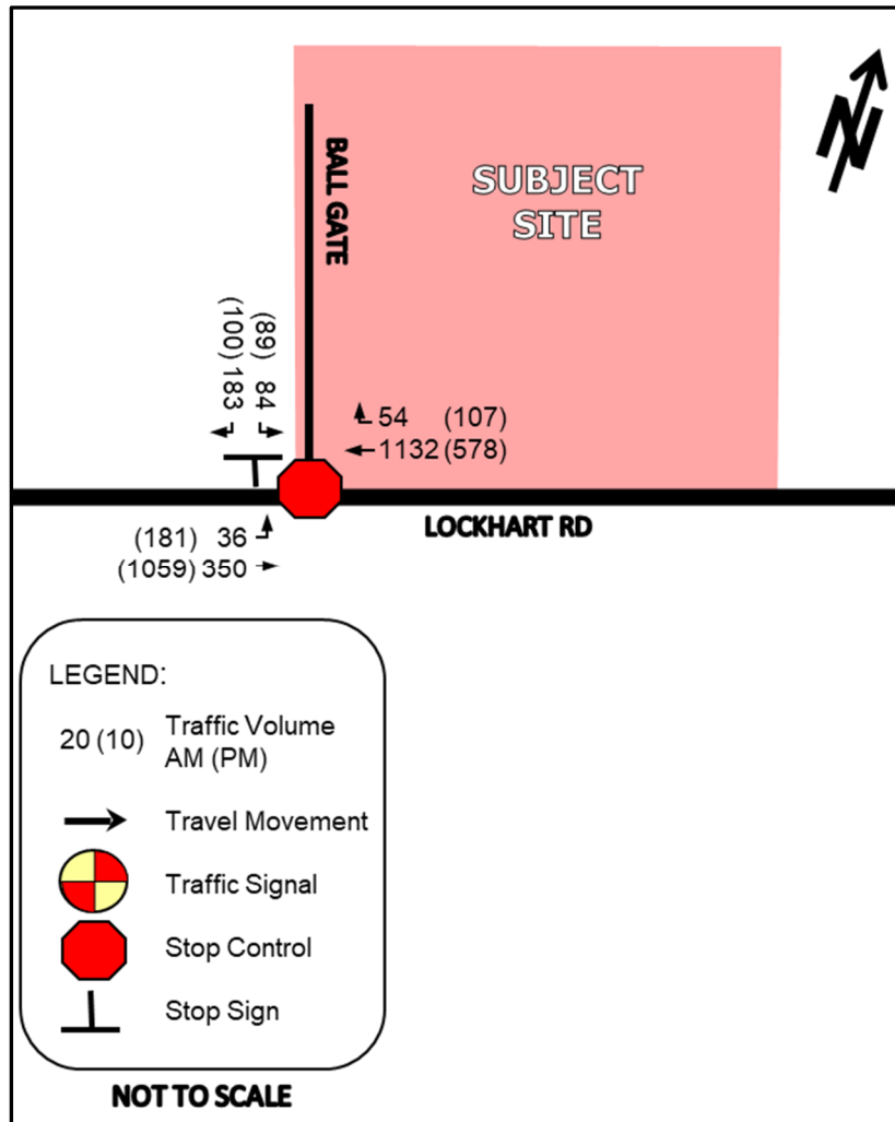
Figure 18 – Total (2035) Traffic Volumes
