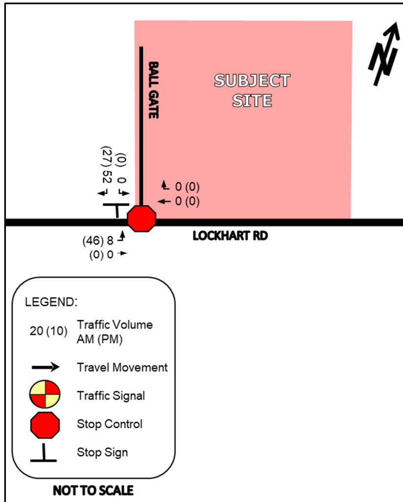
Figure 5 – Lockhart Development P1 Traffic Assignment (2031 / 2035)
