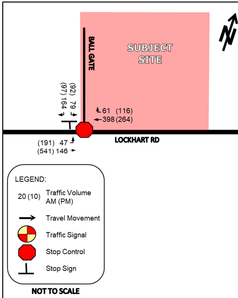
Figure 16 – Total (2025) Traffic Volumes
