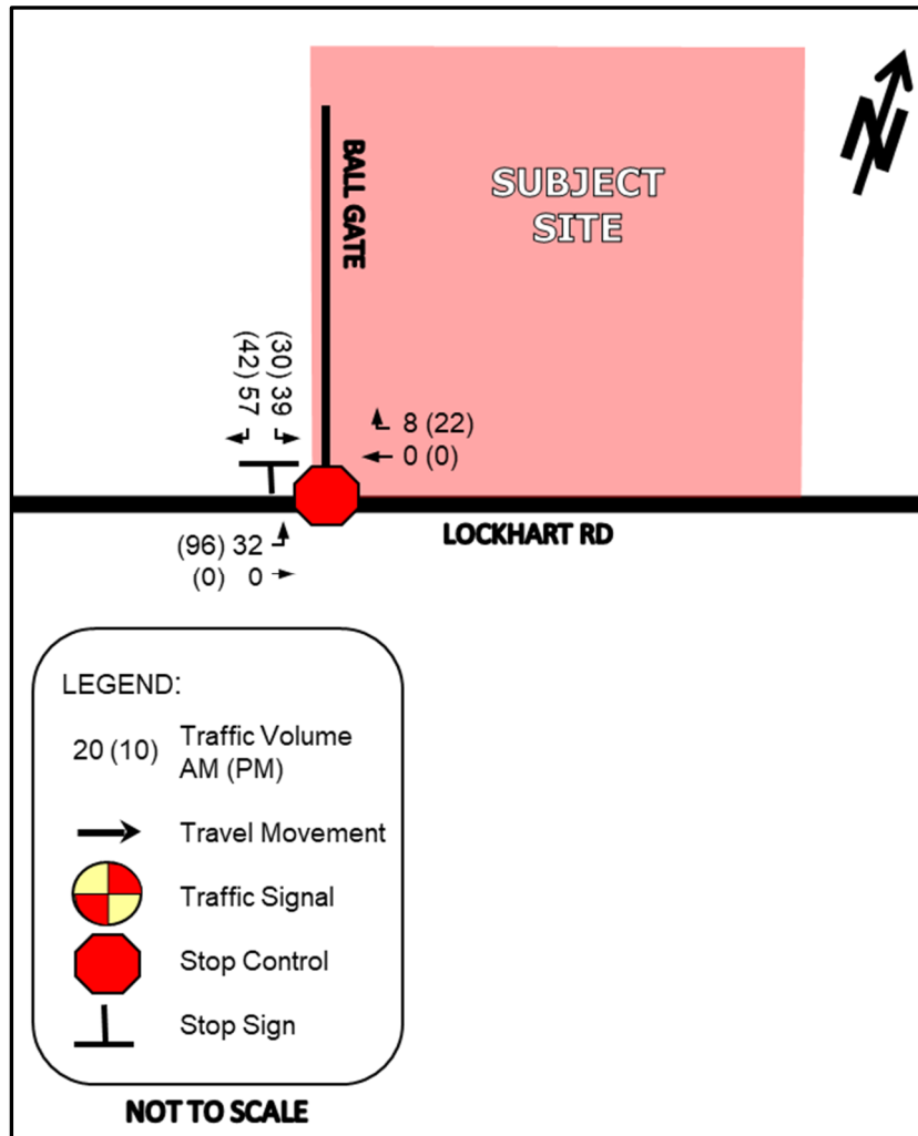
Figure 8 – Sorbara Development Traffic Assignment (2025)
