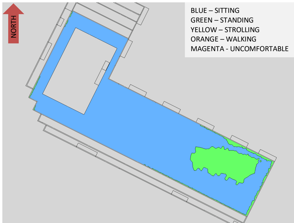
FIGURE 7B: SUMMER – WIND COMFORT, ROOFTOP TERRACE
