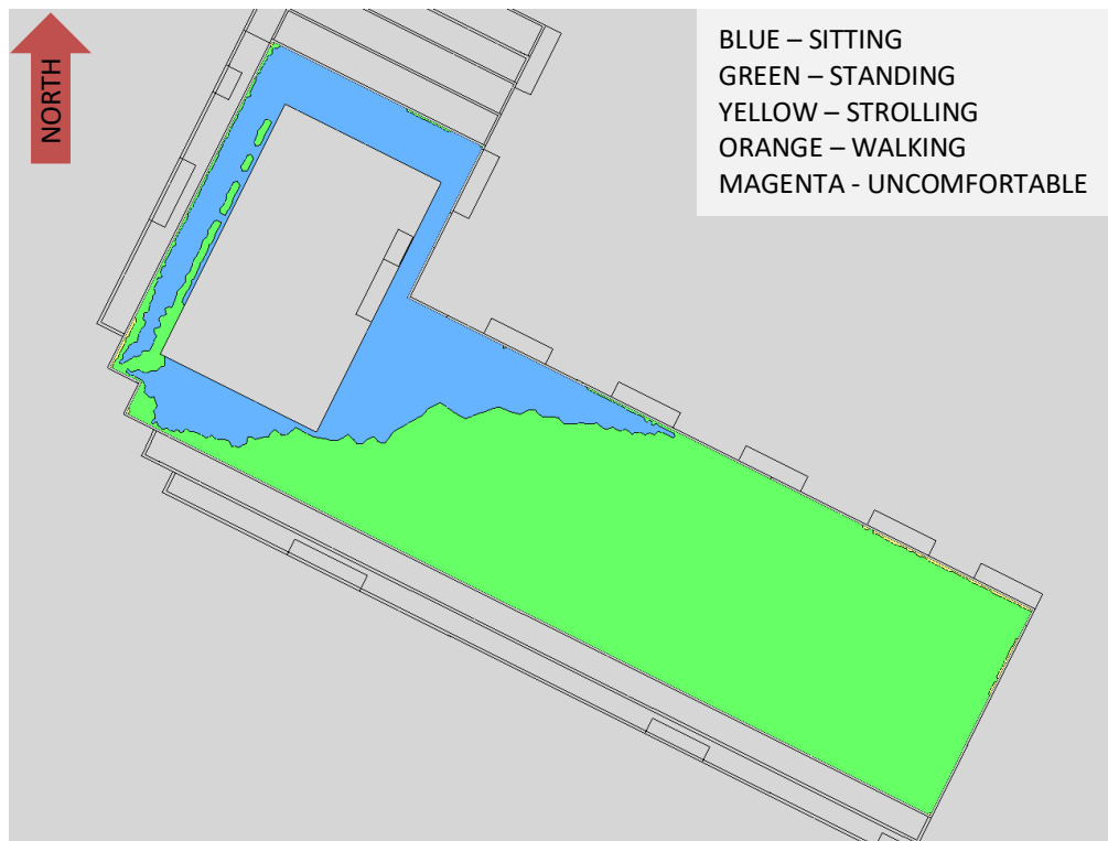
FIGURE 7D: WINTER – WIND COMFORT, ROOFTOP TERRACE
