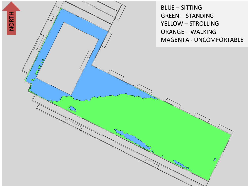
FIGURE 7C: AUTUMN – WIND COMFORT, ROOFTOP TERRACE
