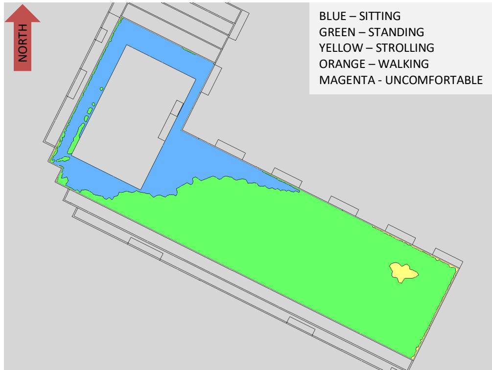
FIGURE 7A: SPRING – WIND COMFORT, ROOFTOP TERRACE
